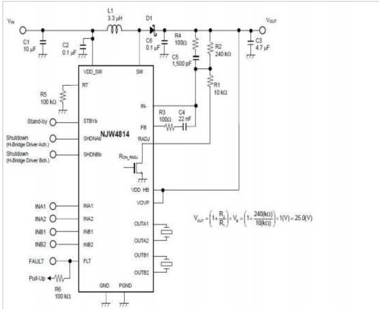
[Figure 5-2] NJW4814 typical application circuit
