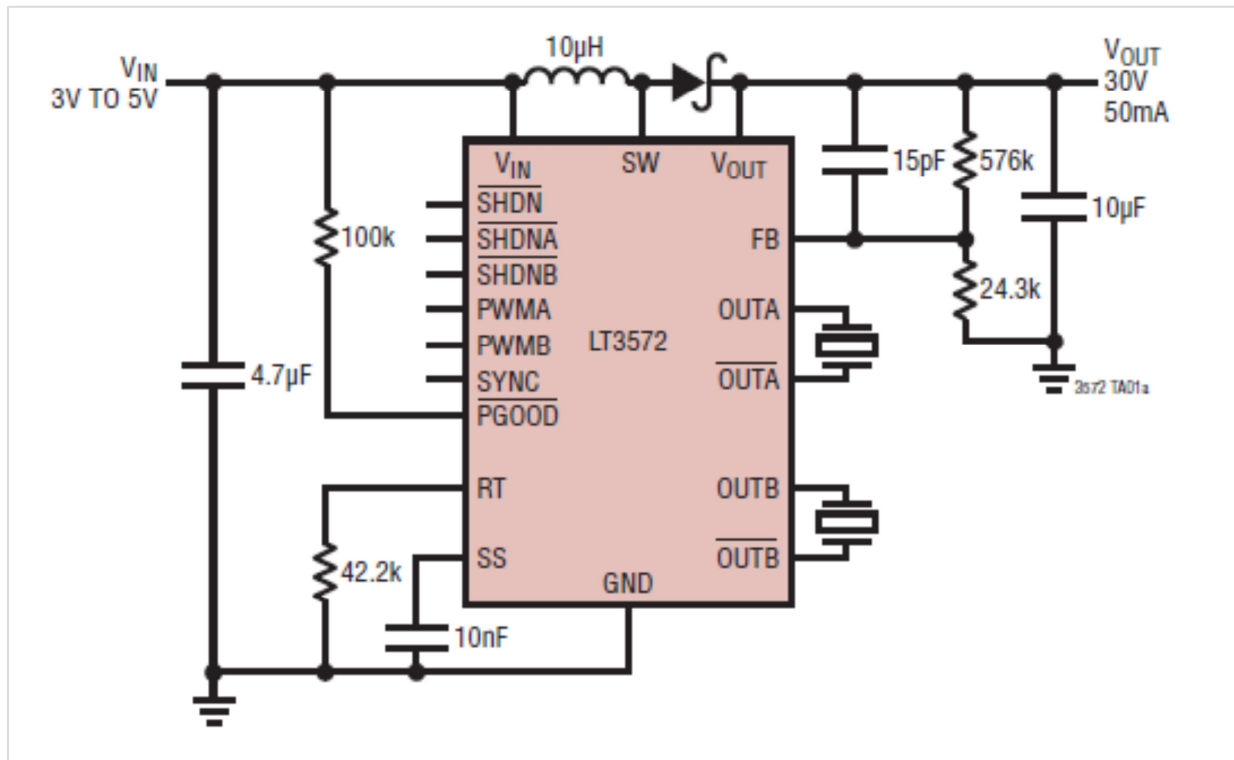
[Figure 5-1] LT3572 typical application
