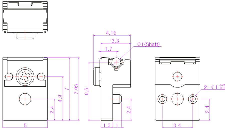
[Figure 4-7] PZM-S-510M Mobile-part (Slider)
