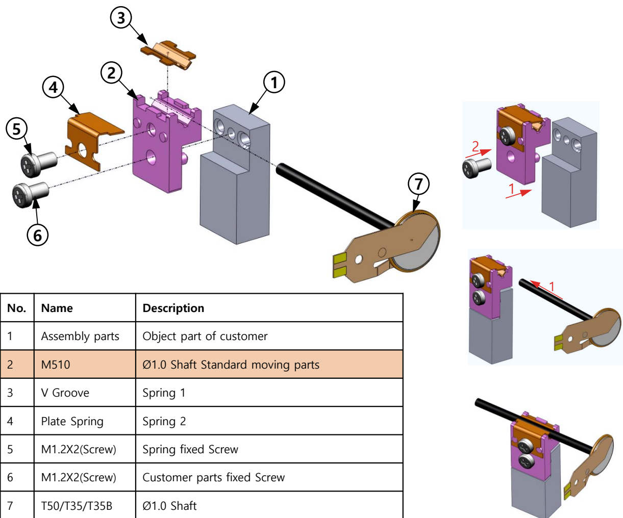
[Figure 4-8] Mounting Steps
